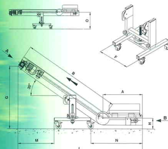
VISTA DA A VIEW FROM A
